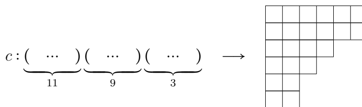
Figure 3.5: Split conjugacy classes and symmetric partitions
