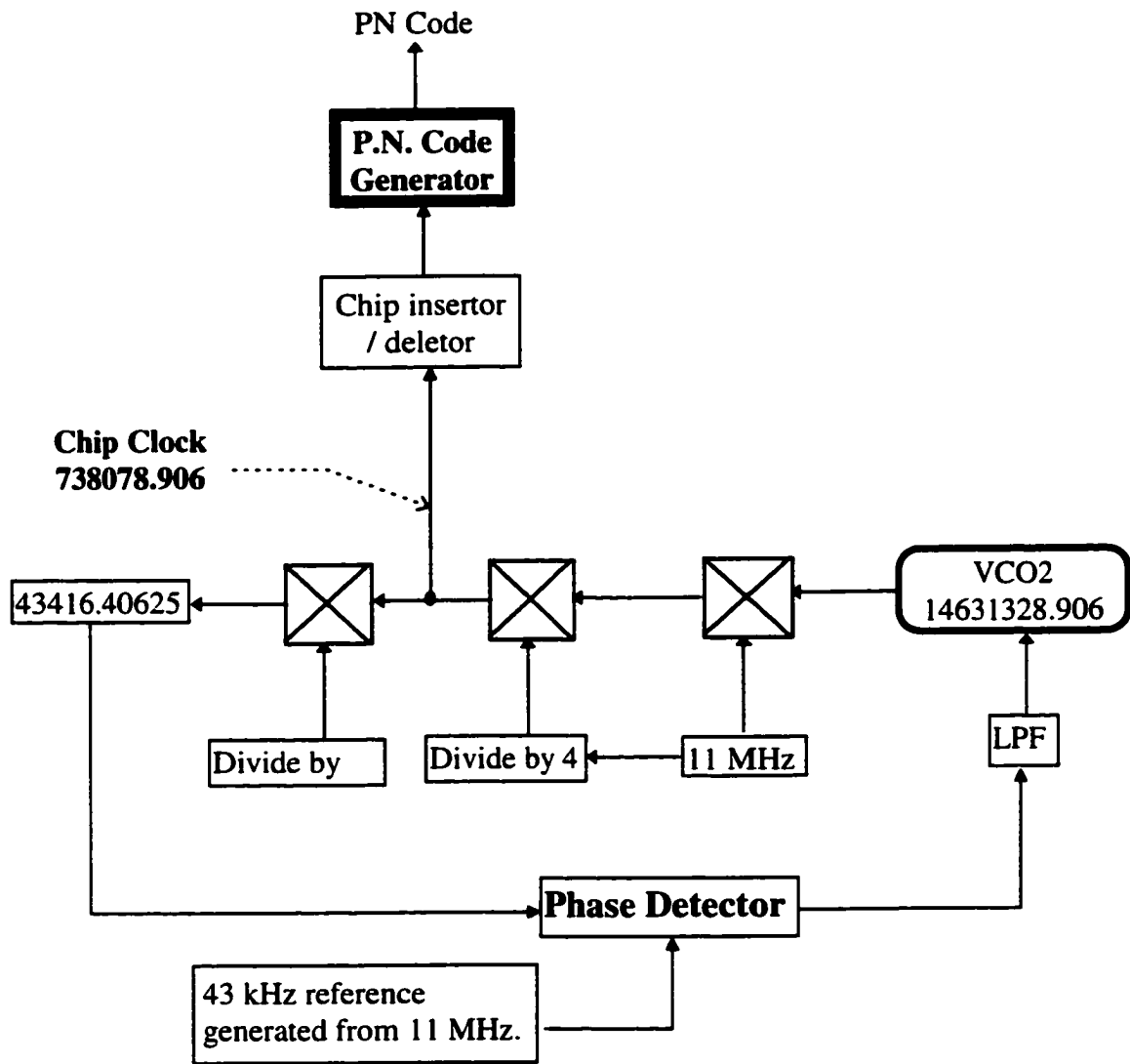
Figure 3.20 Transmit Chip Clock Generation
