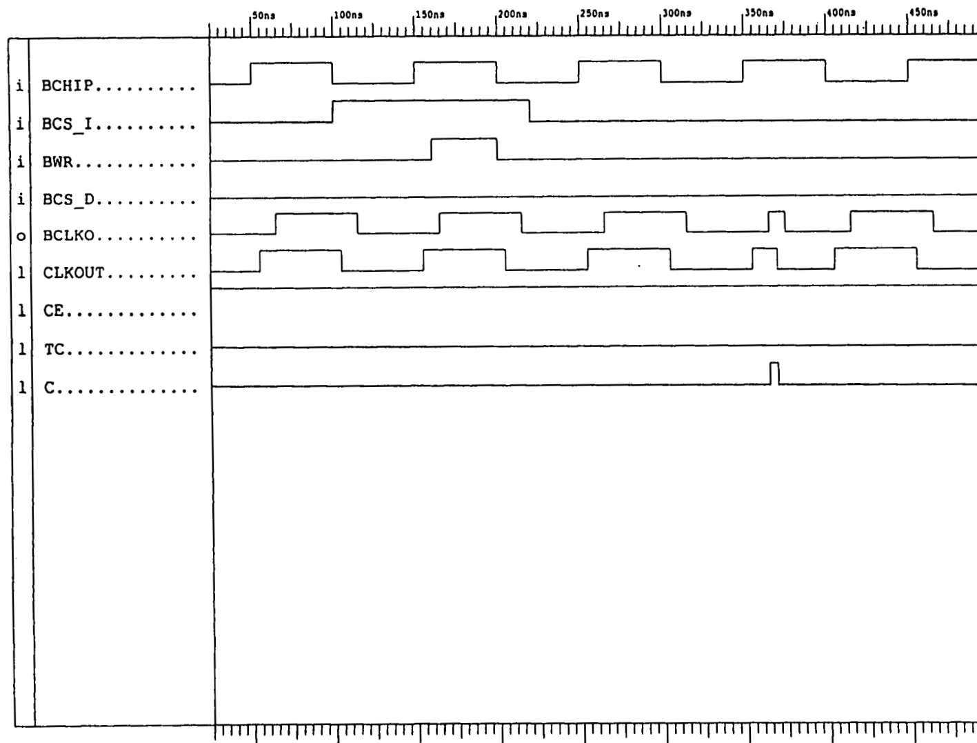
Figure 4.12 Simulation of clock advance.
