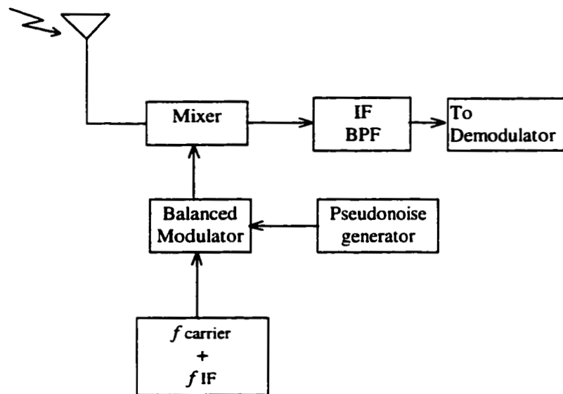
b) Receiver
