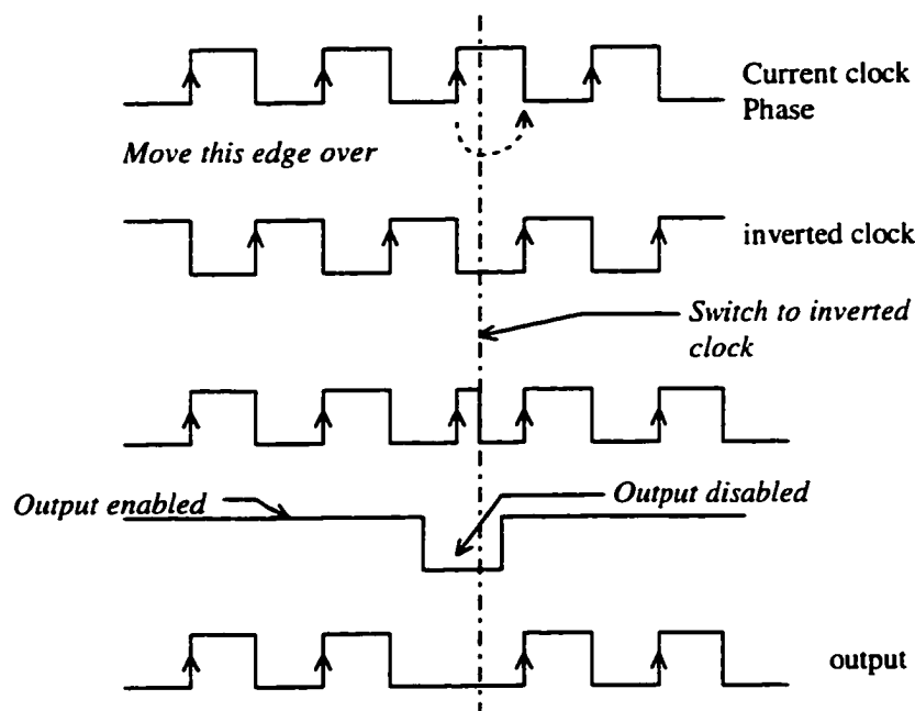
Figure 4.10 Chip deletion / phase retard.
