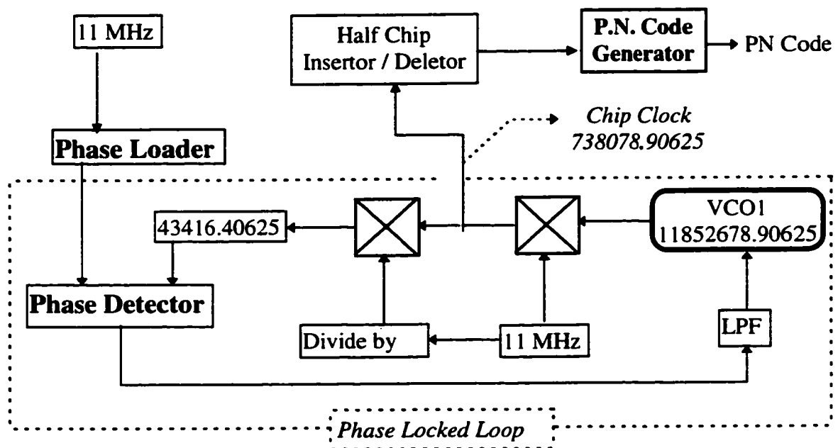
Figure 3.16 PN Code Phase Sliding block diagram.
