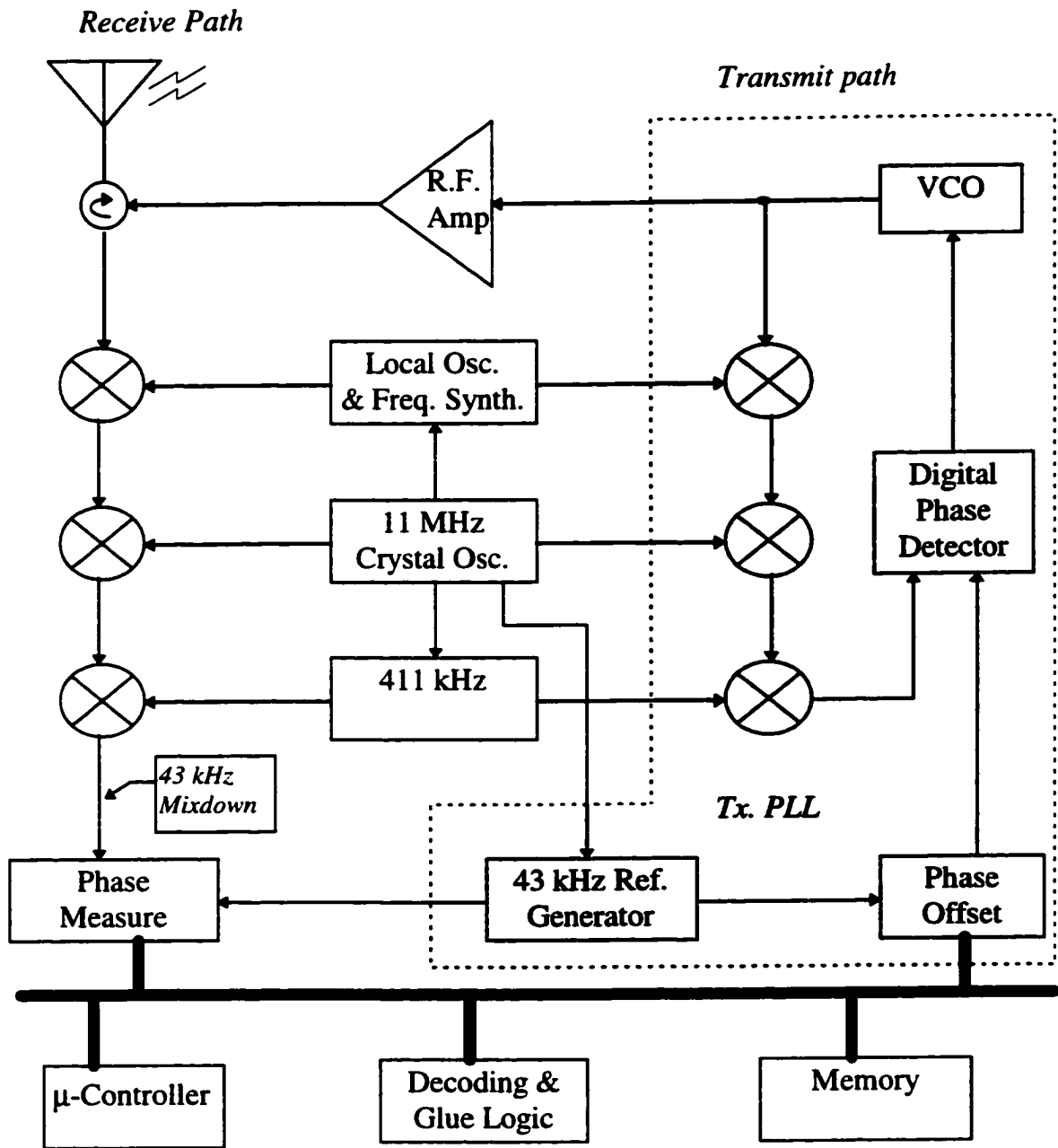
Figure 2.5 Internal block diagram of the beacon in the CWRH system.
