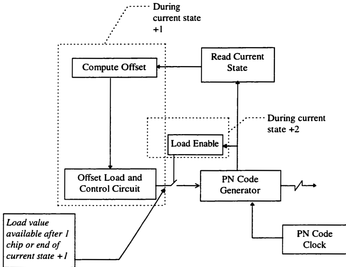
Figure 4.16 Phase Offset Block Diagram.
