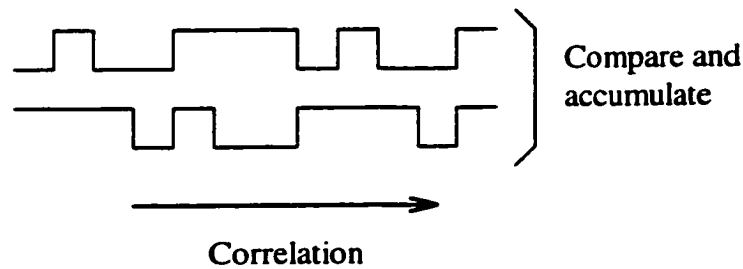
Figure 3.4 Correlation
