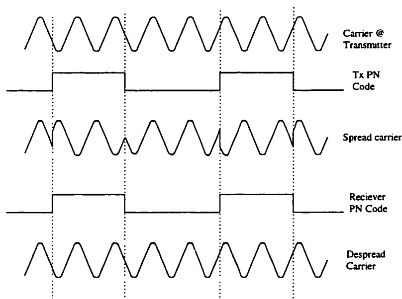
Figure 3.12 Carrier Spreading and Despreading
