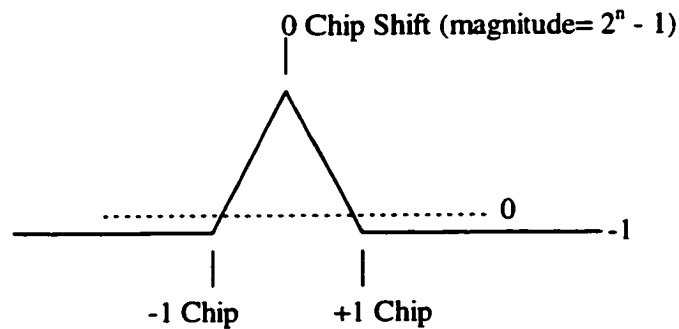
Figure 3.7 Autocorrelation of a maximal sequence
