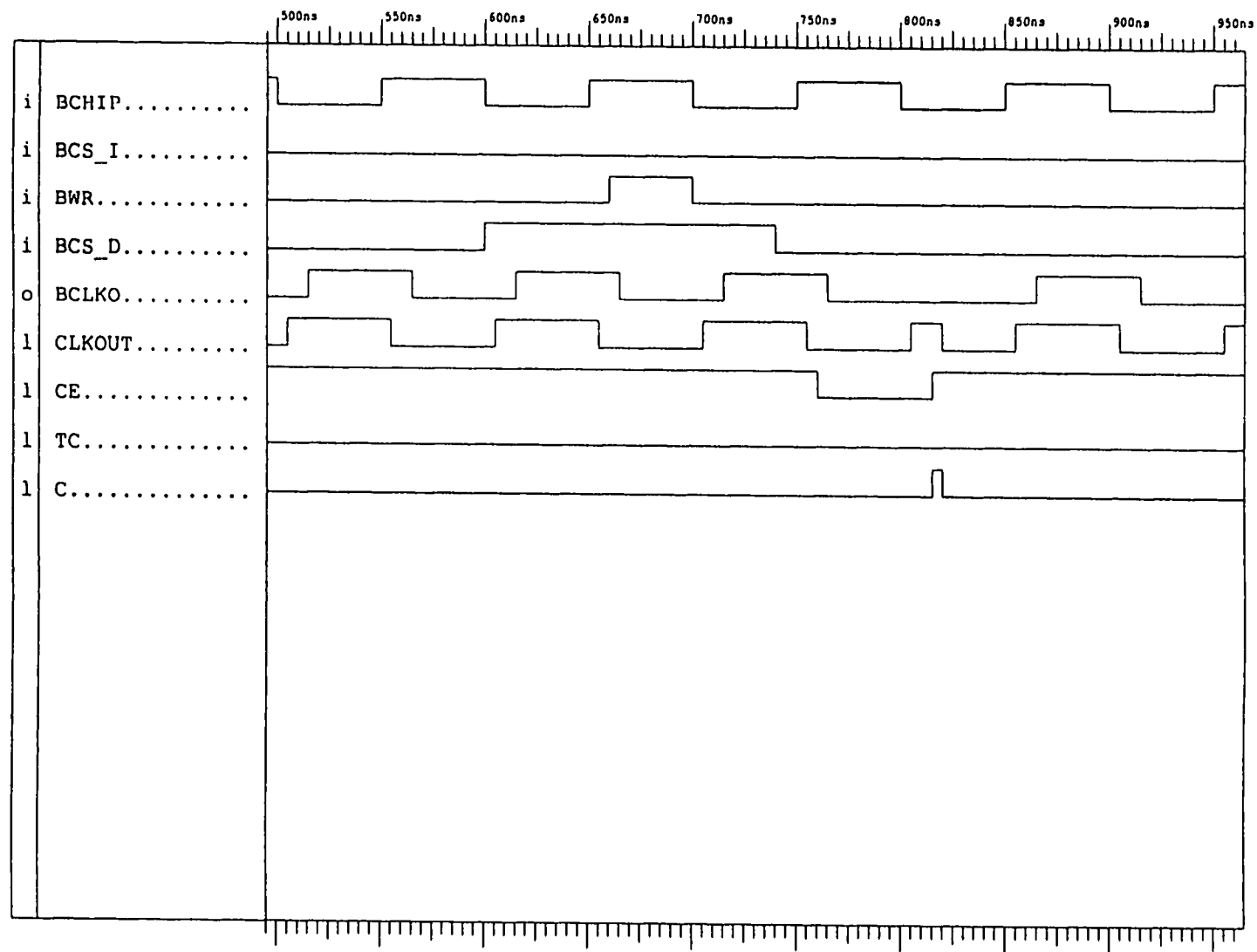
Figure 4.13 Simulation for Clock retard.
