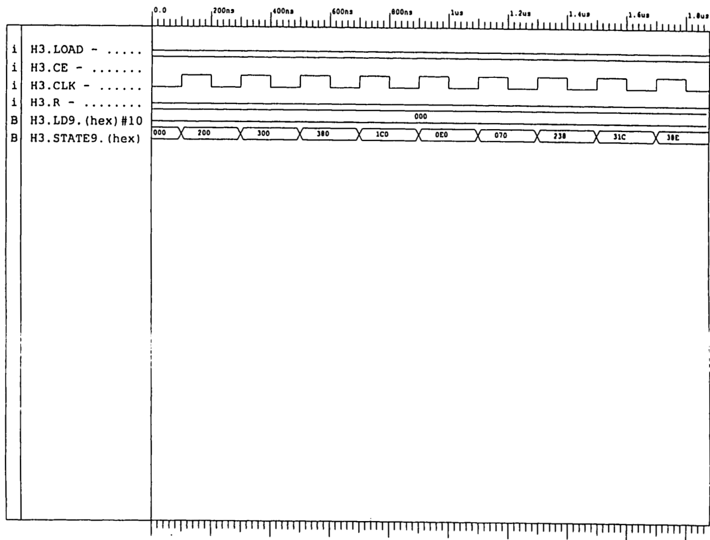
Figure 4.7 Initial simulation of the code generator.
