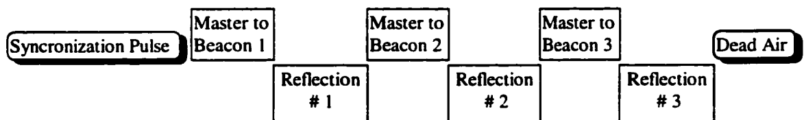
Figure 2.3. Modulation Cycle (87 ms)
